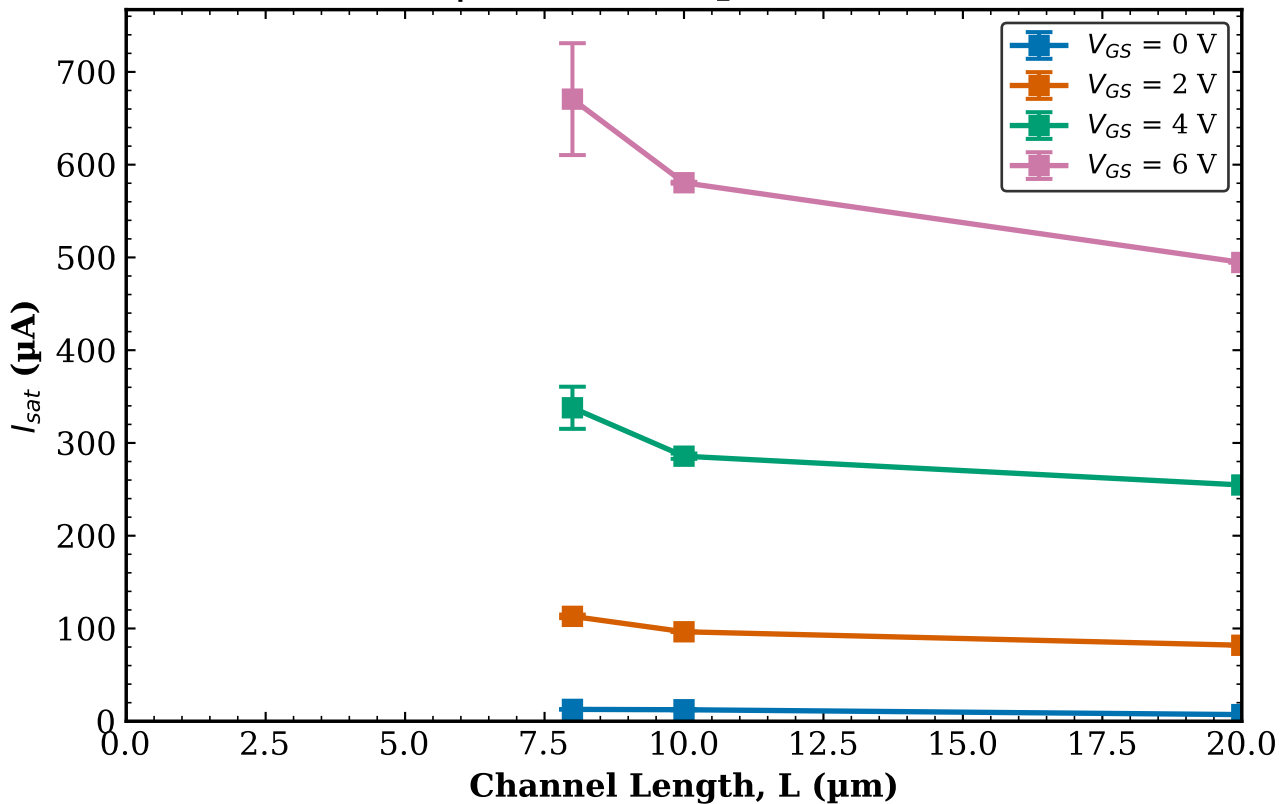
TFT1 Combined (Tr. 1 & 2) I_{sat} vs L | W = 1000 \mu\text{m} (mean \pm std)
